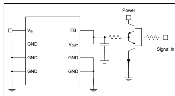
FIGURE 1-1: Long-Term Drift Test Circuit.
