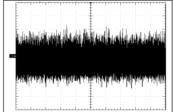
FIGURE 2-22: Noise vs. Time, V_{DD} = 5.5\text{V} , T_A = +25^{\circ}\text{C} , 2.048V Option, No Load, 2\ \mu\text{V/div} , 100\ \text{ms/div} .
